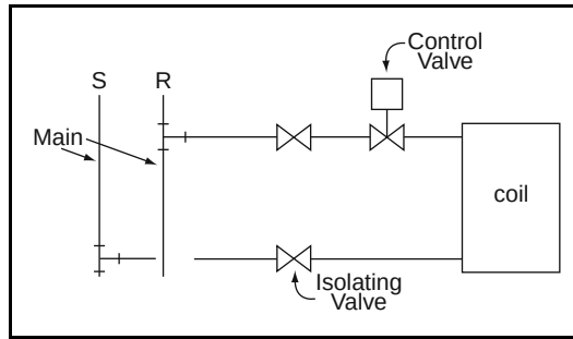
Figure 3-21 Coil Subsystem
