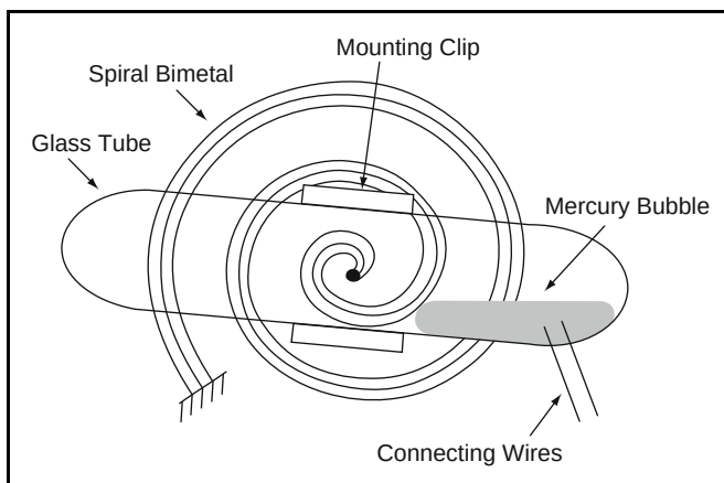
Figure 4-3 Mercury Switch
