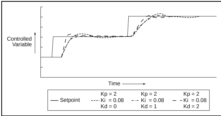
Figure I-17 Proportional-integral-derivative Control
