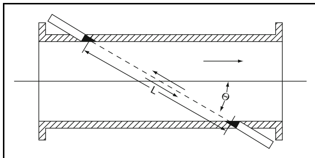
Figure 4-33 Ultrasonic Meter
