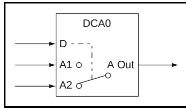
Figure 10-10 DCAO Gate
