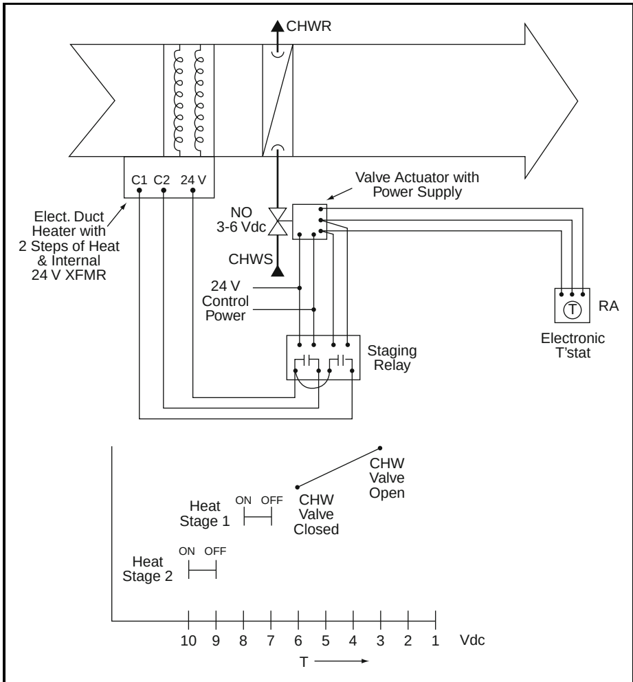
Figure 8-9 Single-zone Unit
