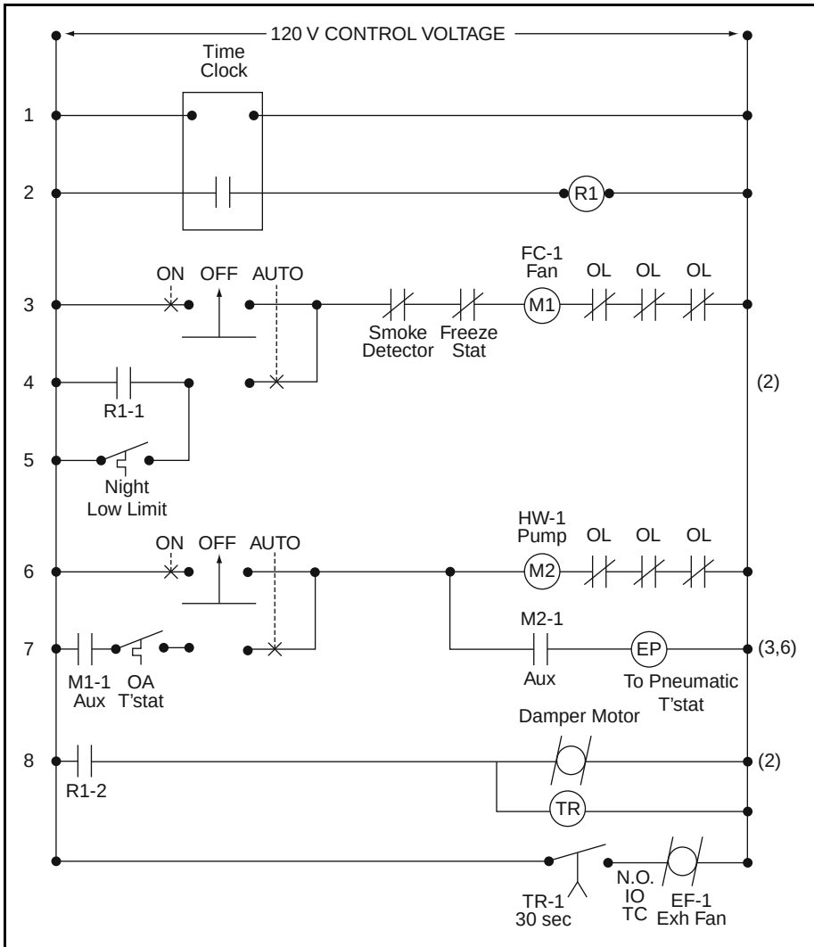
Figure 2-34 Ladder Diagram
