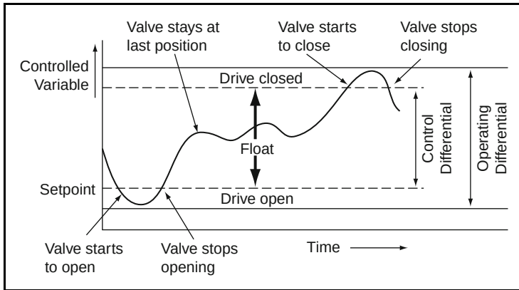
Figure I-8 Floating Control
