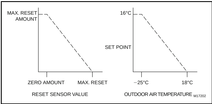
Figure 10-17 Reset Ramp Graph
