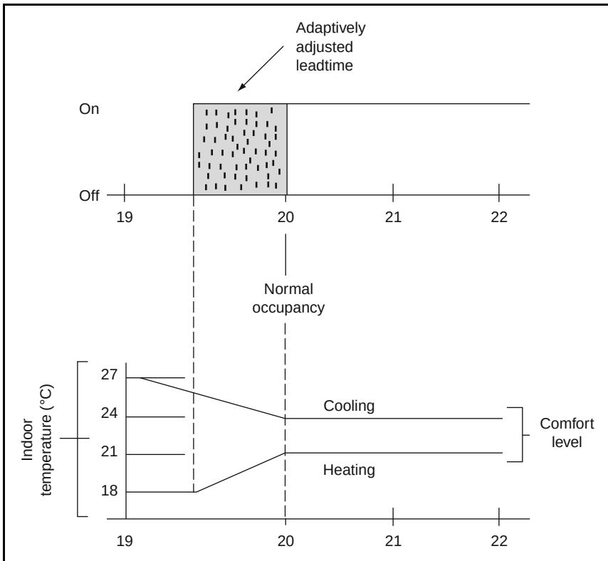
Figure 10-19 Optimum Start
