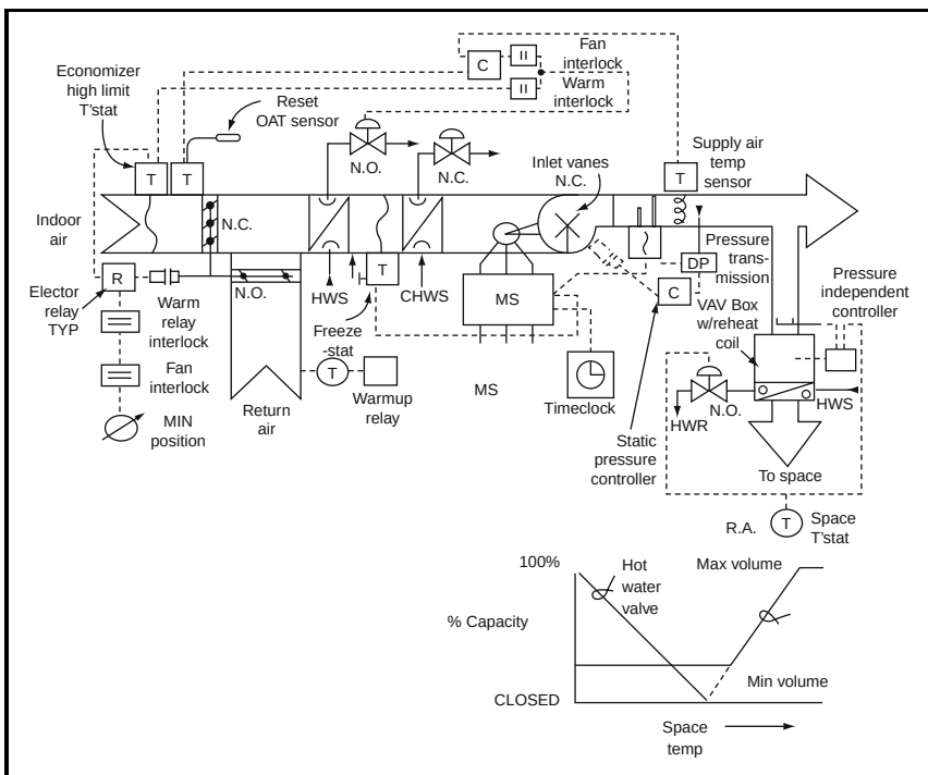
Figure 9-5 Typical VAV Systems AHU
