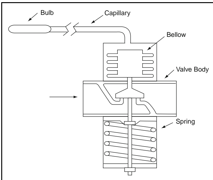
Figure 5-2 Self-powered Valve
