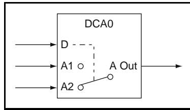
Figure 10-10 DCA0 Gate
