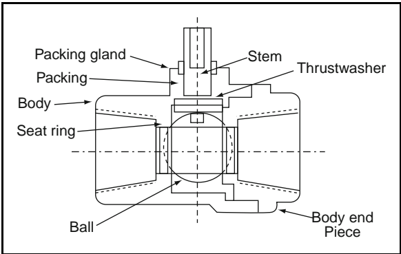
Figure 3-12 Ball Valve Layout
