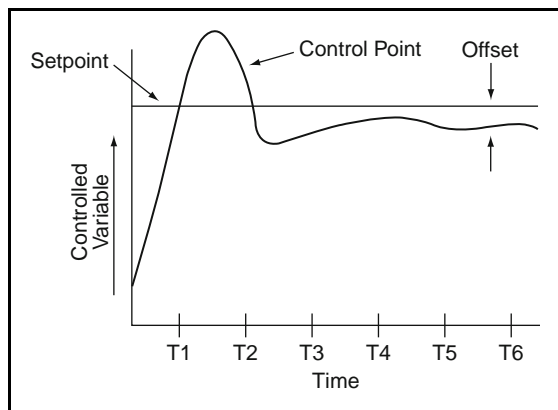
Figure 1-11 Proportional-only Control
