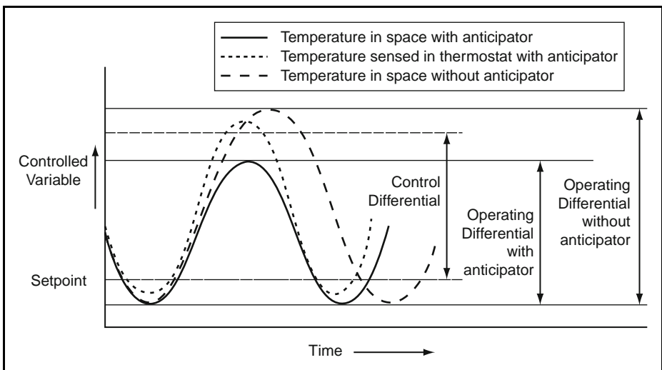
Figure I-6 Two-position Control with Anticipator
