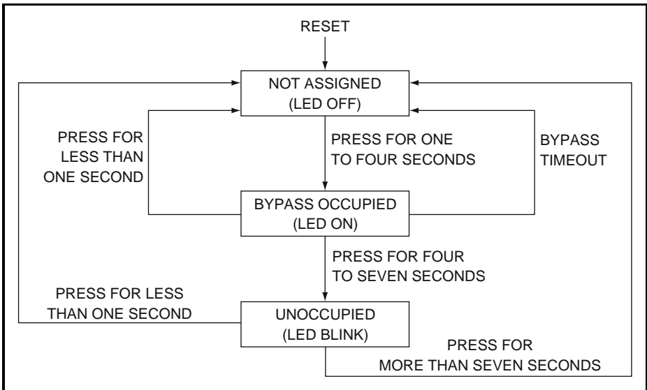
Figure 10-12 Bypass Logic
