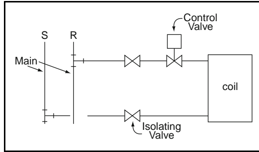
Figure 3-21 Coil Subsystem
