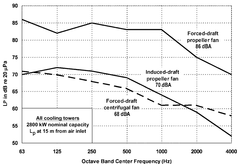
Figure 3-3 ATC-128 octave band L_p values at 15 m from the air inlet side of three types of 2800 kW cooling towers.
