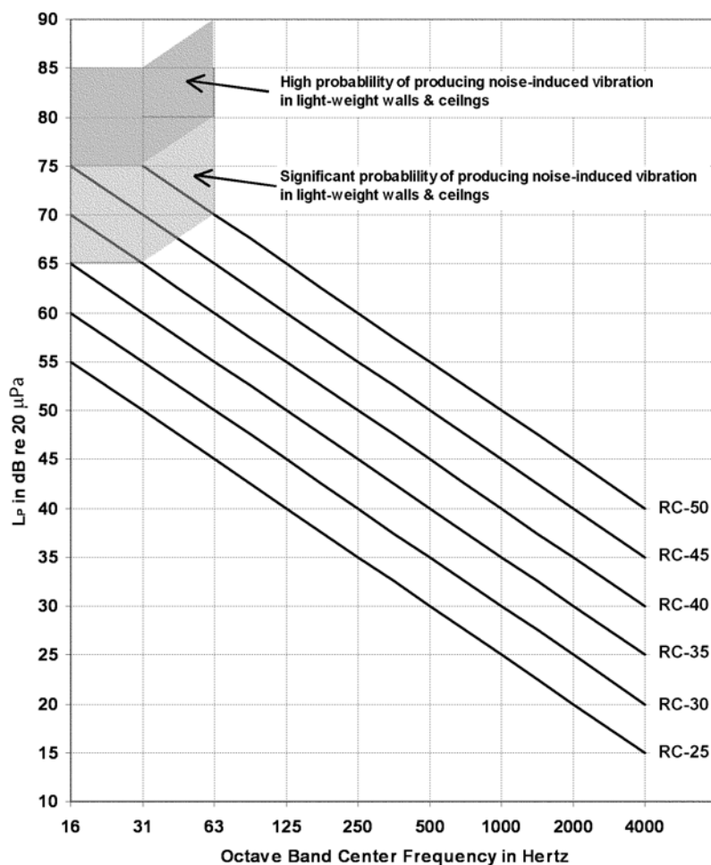
Figure B-2 Blank RC chart.
