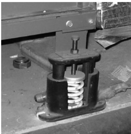
Figure 8-4 Restrained spring isolator with a “short circuit” between its baseplate and equipment mounting plate. This type of isolator has become obsolete and is not recommended for any type of HVAC equipment.
