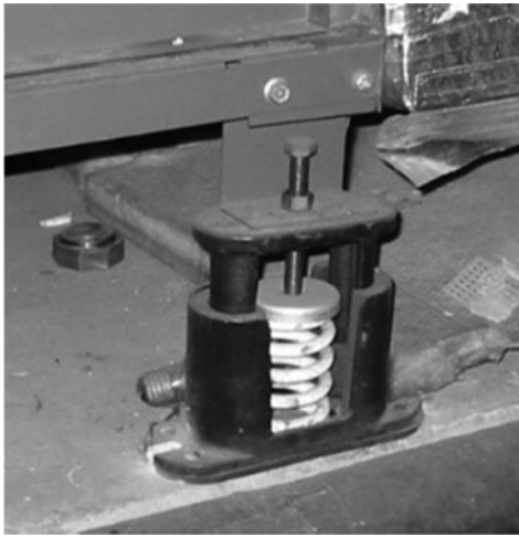
Figure 5-8 Cast-metal floor mount is prone to “short-circuiting” and should never be used. Instead, use a floor mount like that shown in Figure 5-6.
