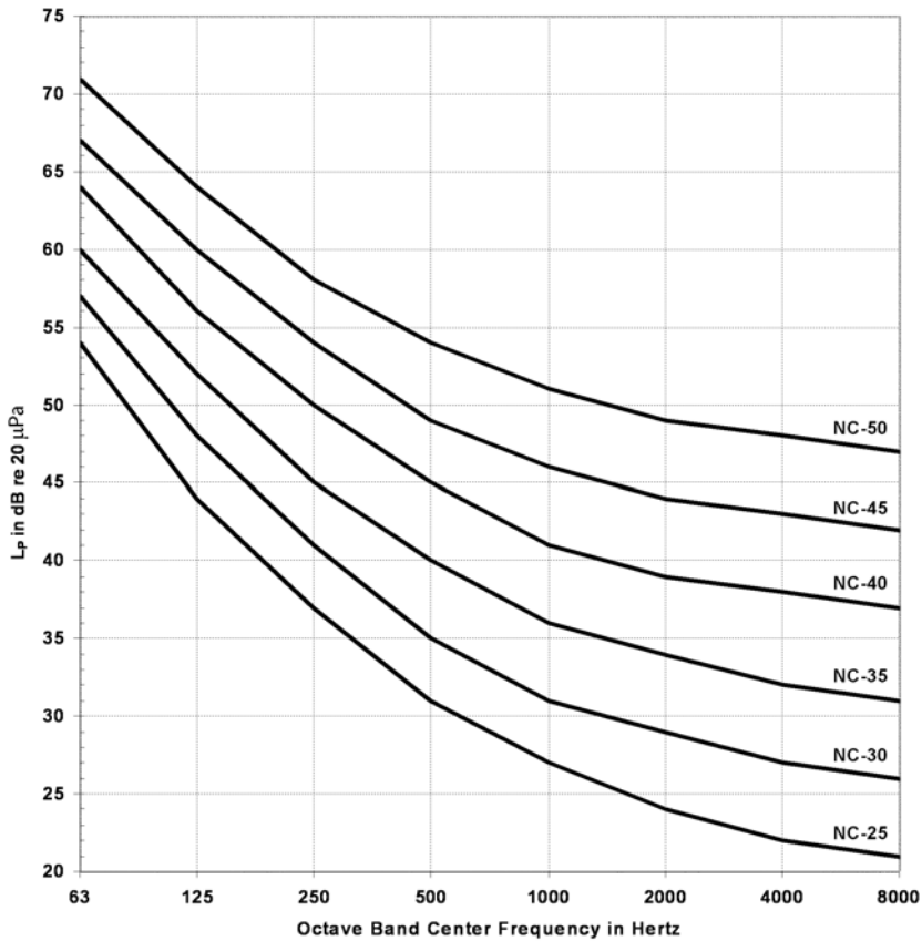
Figure B-4 Blank NC chart.
