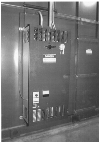
Figure 2-52 Variable-frequency drive.
