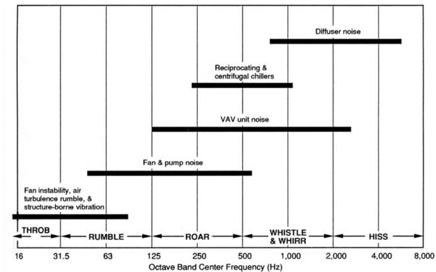
Figure A-5 Frequencies at which various types of HVAC equipment generally control their sound spectra.
