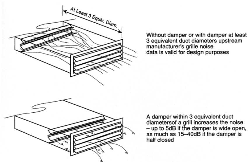
Figure 2-26 The effect of installing a damper behind a grille.
