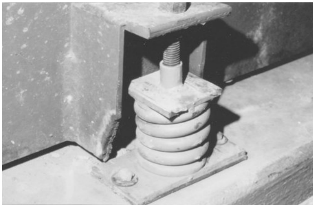
Figure 7-6 Overloaded free-standing floor mount. The overloading allowed the gussets welded to the side of the equipment frame to rest on top of the isolator baseplate. The lower right corner of the gusset was burned off to eliminate the gusset/baseplate contact. The proper action would have been to replace the overloaded spring with a stiffer one able to carry the heavy load.
