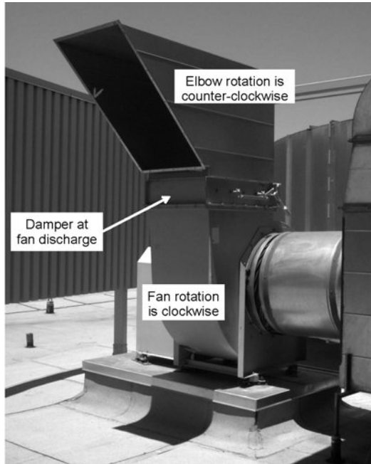
Figure 8-3 Fan installation with poor discharge duct system aerodynamics. The close-coupled discharge damper and reverse-direction elbow create extremely high turbulence that creates rotating fan stall, performance reduction, and rumble.
