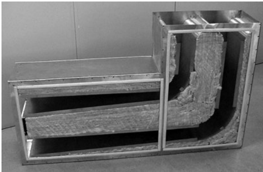
Figure 2-41 Cutaway view of an elbow duct silencer.
