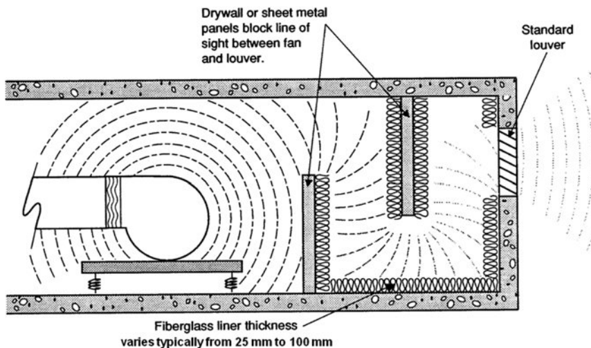
Figure I-5 Labyrinth air path used for sound attenuation at an equipment room ventilation opening.
