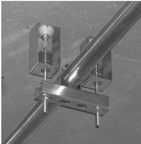
Figure 5-5 Spring hanger installation with proper spring compression and hanger rod centered through hole at bottom of hanger box.
