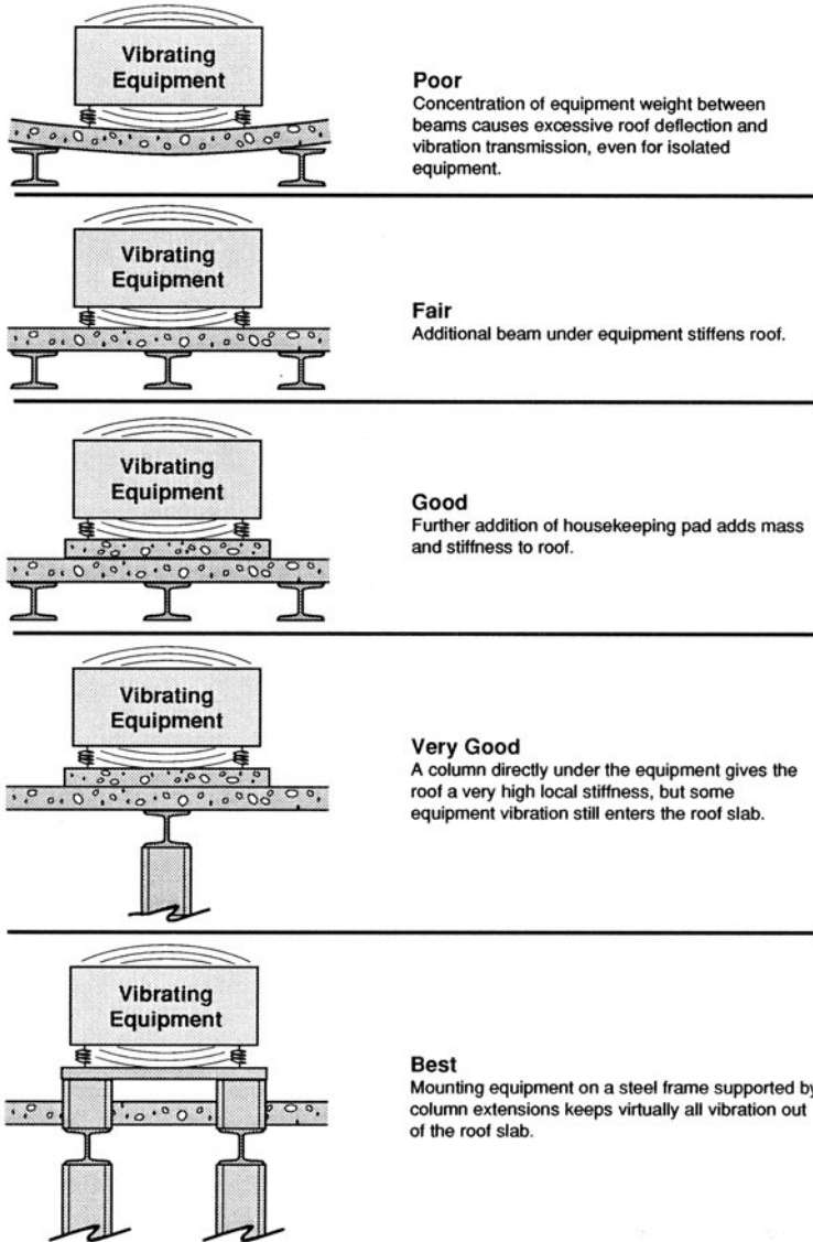
Figure I-16 Structural support of rooftop equipment for vibration control.
