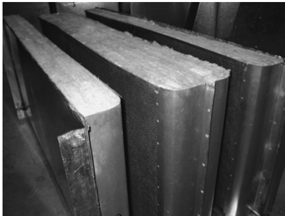
Figure 2-38 Cutaway view into a dissipative duct silencer.
