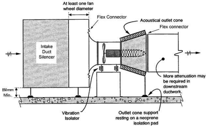
Figure 1-14 Typical duct silencer arrangement at vane-axial fan.
