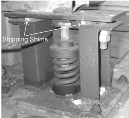
Figure 7-7 Short-circuited floor mount isolator whose shipping shims have not been removed.
