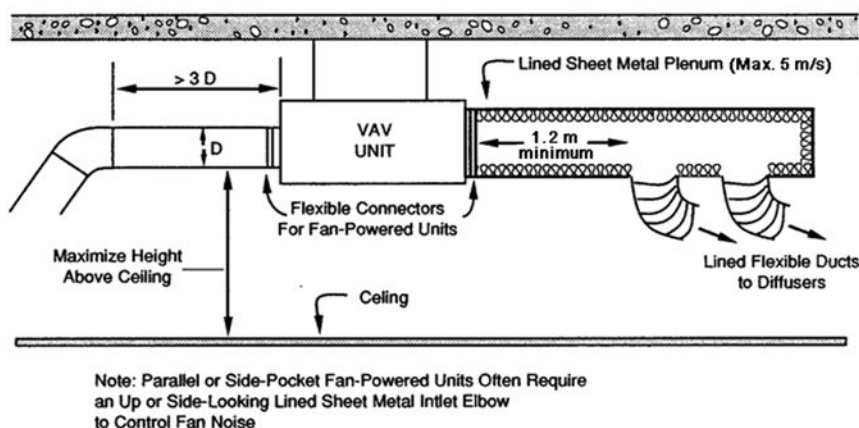
Figure 2-22 Guidelines for VAV unit installation.
