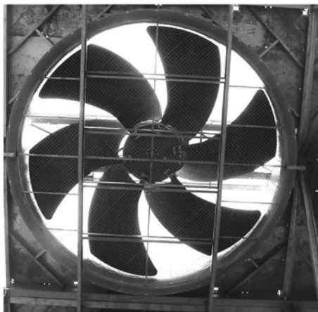
Figure 3-6 View of an induced-draft fan with wide-chord blades. This fan type can be as much as 12 dBA quieter than a “standard” fan of the same diameter.
