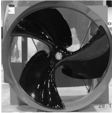
Figure 2-15 Ultra-low-noise propeller fan with backswept airfoil blades. Versions of this fan are available with 2, 3, or 4 blades of adjustable blade twist and diameters up to 12.3 m for very large capacities.
