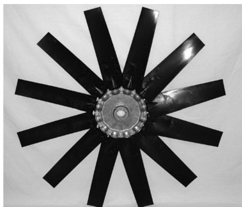
Figure 2-14 Propeller fan with a 12-socket aluminum hub and plastic blades. This fan can be selected for use with 2, 3, 4, 6, 8, 9, or 12 blades of any custom length or blade twist to optimize airflow and acoustical performance.
