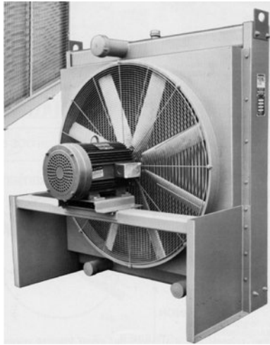
Figure 4-12 Remote radiator for engine-generator sets can be quiet with an oversized, variable-speed cooling fan.
