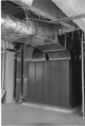
Figure 2-20 Plenum AHU with supply ducts attached to the top of discharge plenum.
