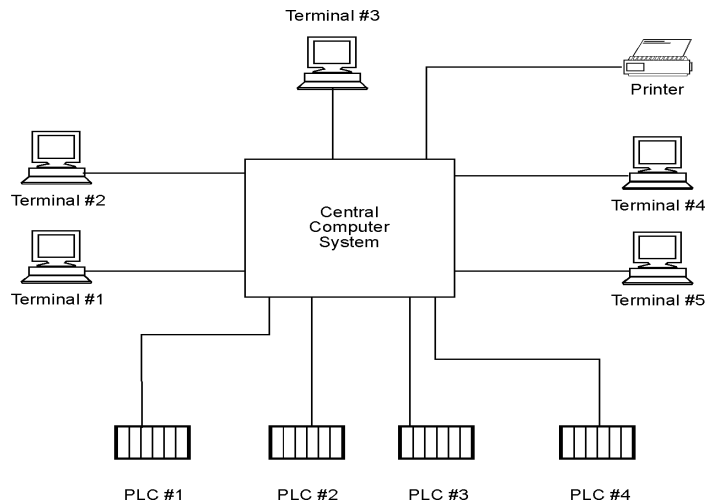
Figure 3.2 Centralized processing
