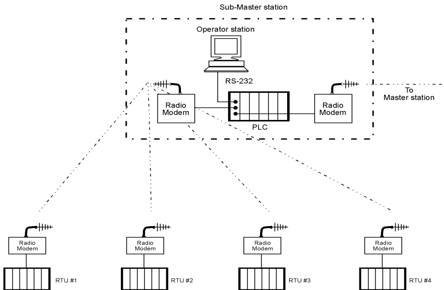
Figure 2.30 Submaster architecture
