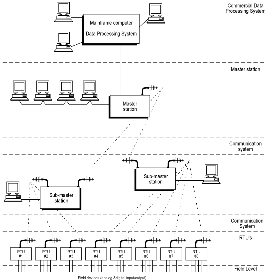
Figure 2.2 SCADA system
