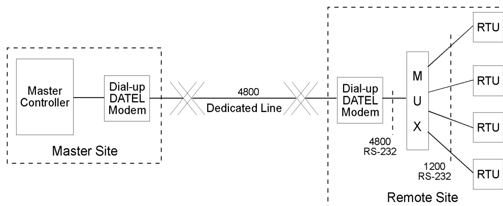
Figure 4.29 DATEL point-to-multipoint connection with multiplexer
