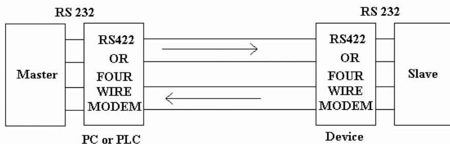
Figure 3.18 Four wire direct mode
