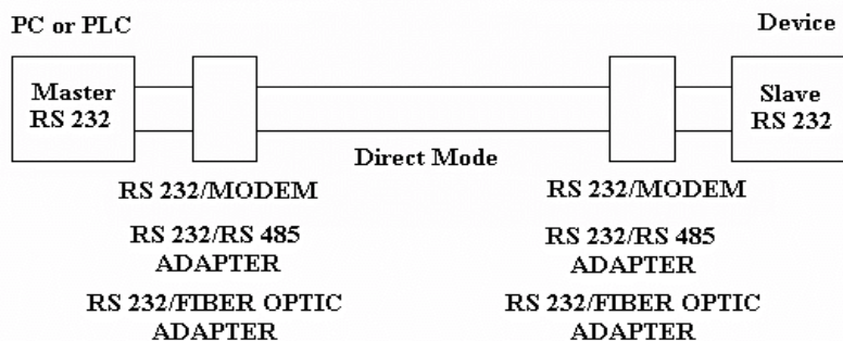
Figure 3.16 Two wire direct mode
