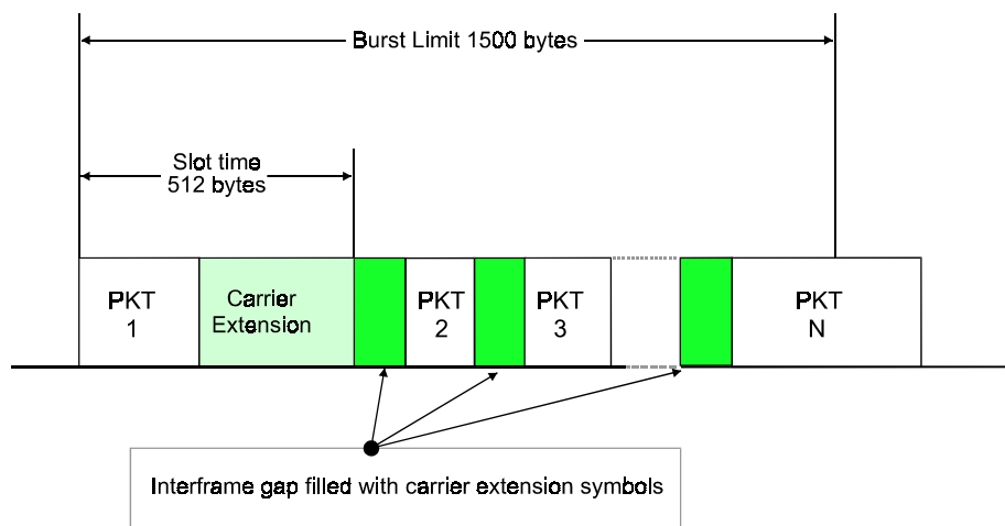
Figure 5.14 Packet bursting
