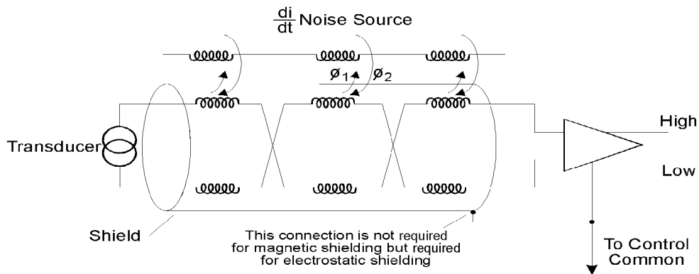
Figure 4.7 Effects of shield in reducing magnetic coupling
