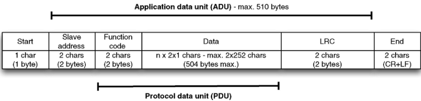
FIGURE 6.5 Modbus frame (Modbus ASCII).
