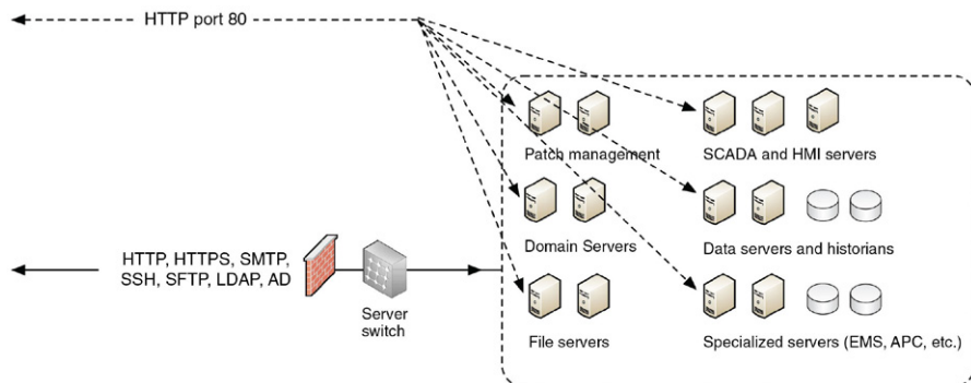
FIGURE 2.10 Placing all services behind a common defense provides a broader attack surface on all systems.
