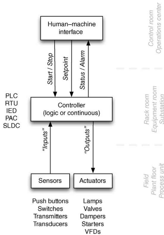
FIGURE 4.6 Human-machine interface functionality.
