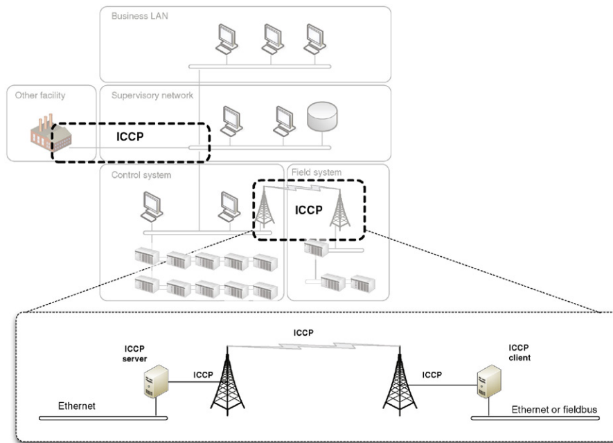
FIGURE 6.25 Typical ICCP use within the industrial network architecture.
