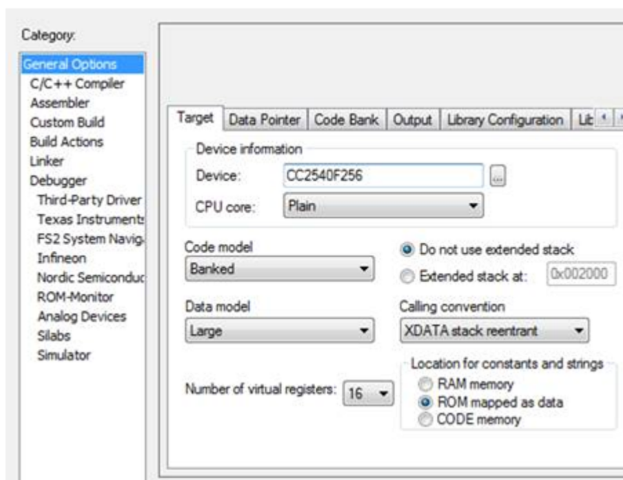
Figure 9-2. IAR Project Options - Device Selection
