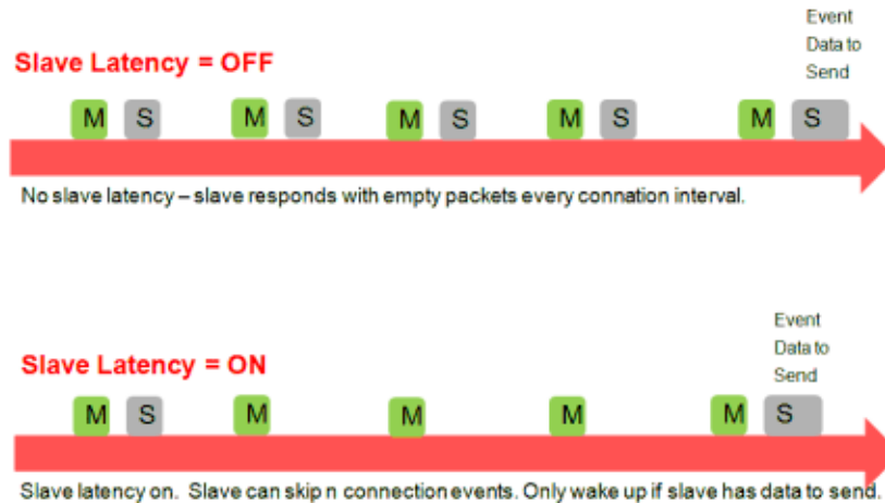
Figure 5-3. Slave Latency
