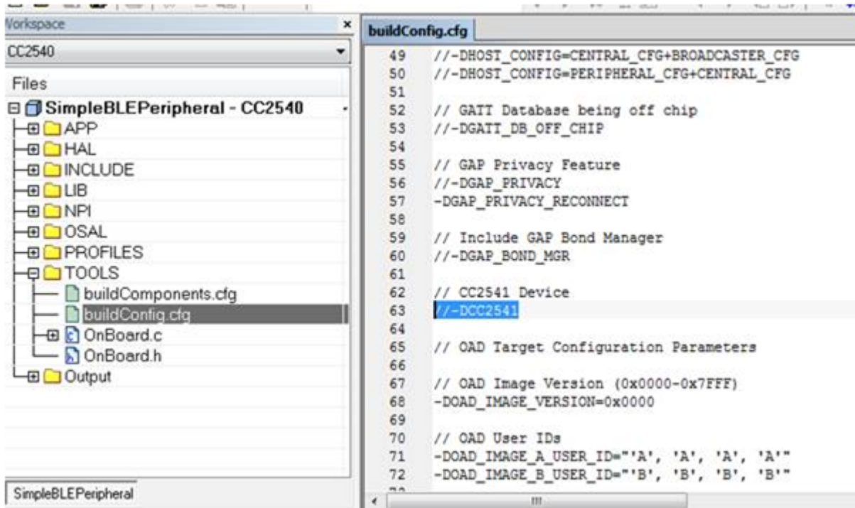
Figure 9-4. Stack Build Configuration
