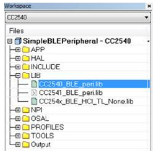
Figure 9-6. BLE Library: Add To LIB Group
