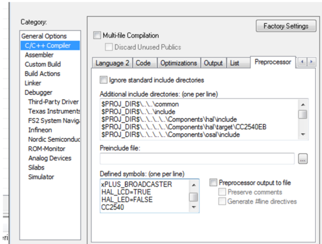
Figure 9-3. IAR Project Options - Predefined Symbols
