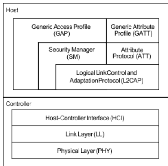
Figure 1-1. Bluetooth Low Energy Protocol Stack
