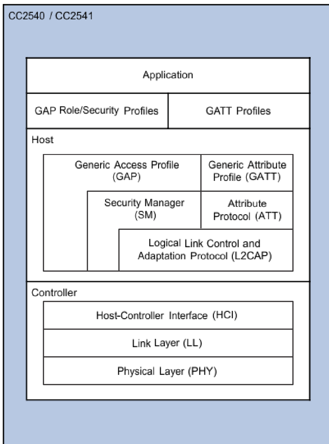
Figure 2-1. Single-Device Configuration
