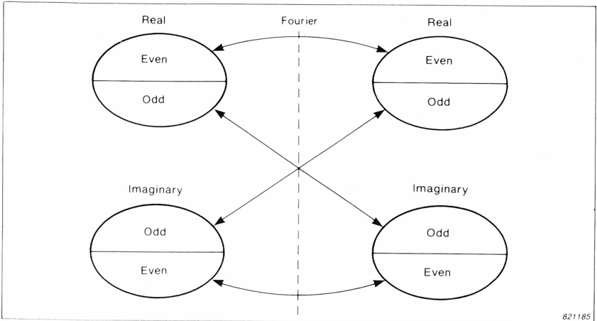
Fig. 2.2. The separation of a function in real and imaginary, even and odd parts is often convenient. Use of the relationships indicated in the figure facilitates Fourier Transform calculations by replacing complex and infinite integration with real and semi-infinite integration
