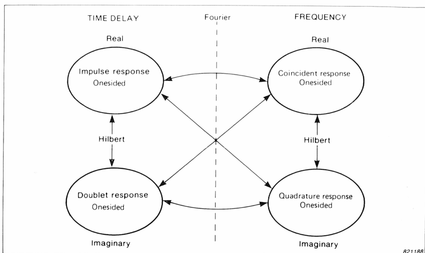
Fig. 3.5. The analytical response is complex but one-sided in both domains. From any of the four partial representations the other three can be derived
