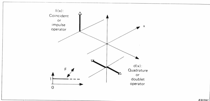
Fig. 2.6. Tending towards a semi-infinite frequency or time range the projections of the Fourier Transform approach the idealized operators \delta(x) and d(x)
