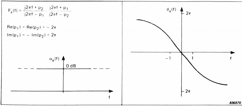
Fig. 3.11. Frequency response of a simple allpass system. The phase will always decrease monotonously with frequency
