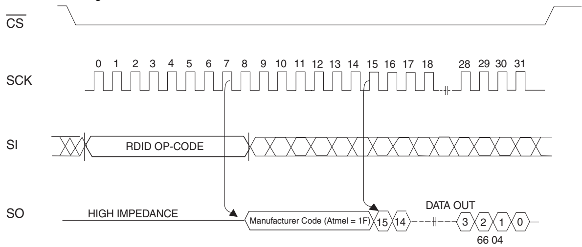
Figure 5-13. RDID Timing
