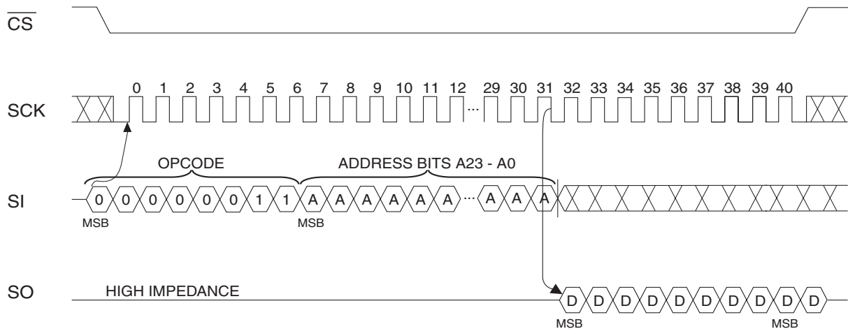
Figure 5-6. READ Timing
