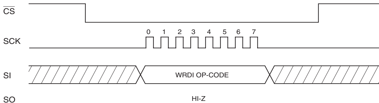
Figure 5-3. WRDI Timing
