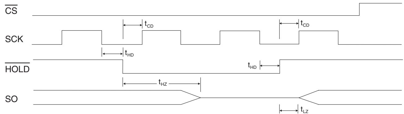
Figure 5-9. HOLD Timing
