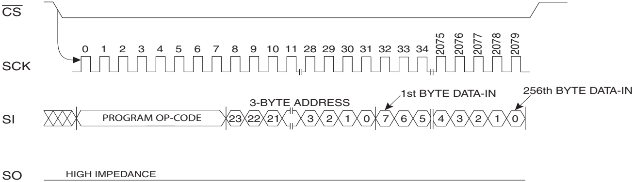
Figure 5-8. PROGRAM Timing
