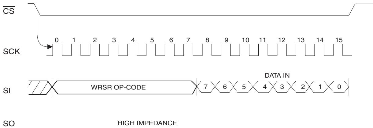
Figure 5-5. WRSR Timing
