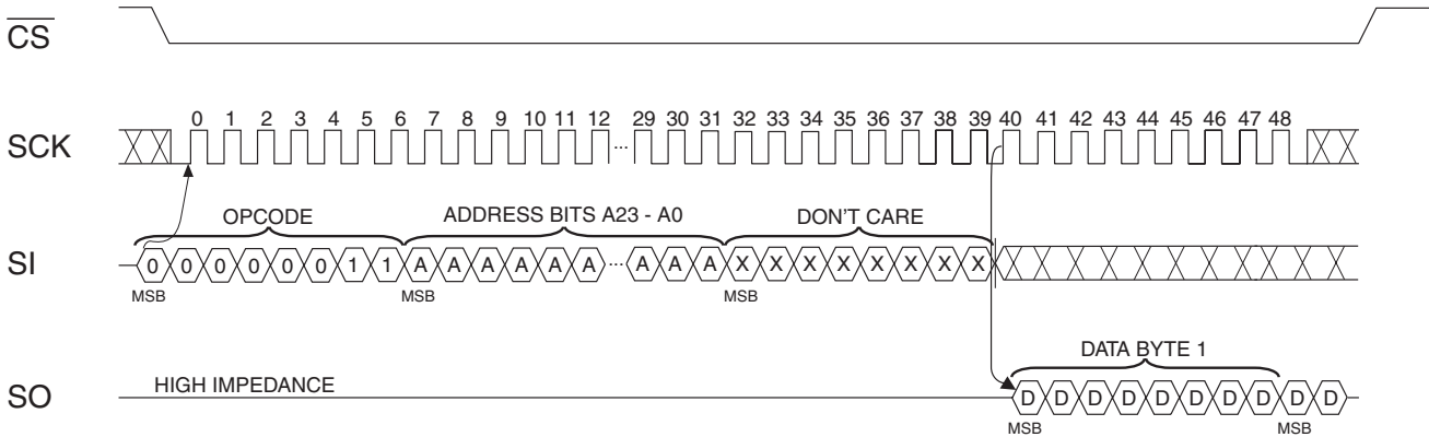
Figure 5-7. FAST READ Timing
