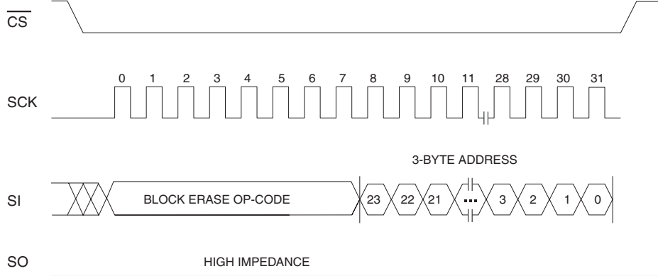
Figure 5-11. BLOCK ERASE Timing
