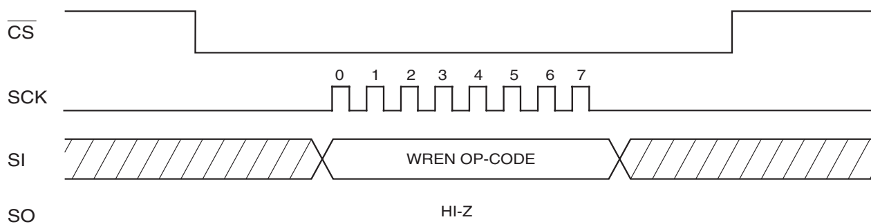
Figure 5-2. WREN Timing
